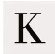
Letter K
